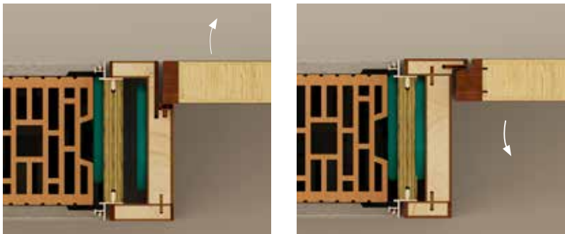
Detail Zarge: SLIM-IN 2.0
